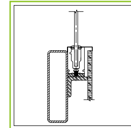
Fascia Mount
