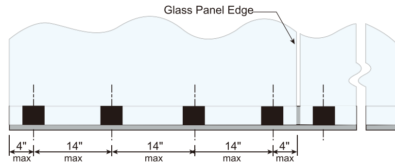
Top Mount
