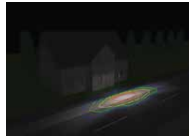
Distribution Type II (T2)
