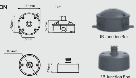
SB Junction Box
